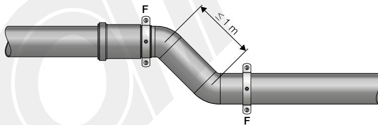
Figure 7.24 Anchor points on deviations smaller than or equal to 1 m (for HDPE).
