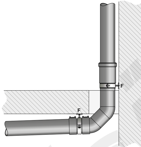
Figure 7.20 Anchor point with a guide bracket and two electrofusion sleeves (for HDPE).
