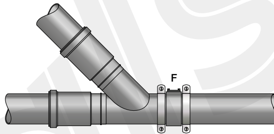
Figure 7.21 Anchor point with two guide brackets and an electrofusion sleeve (for HDPE).
