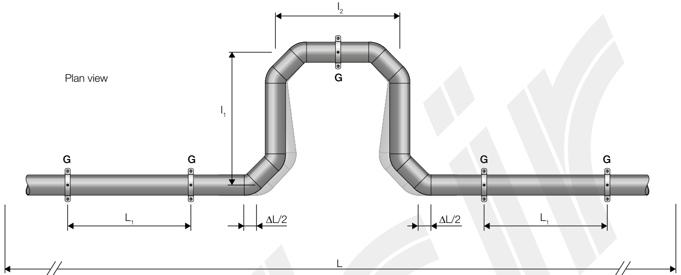
Figure 7.54 “Omega” compensation Type U (for HDPE).
