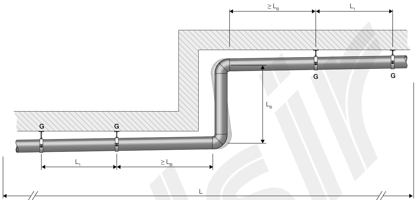
Figure 7.52 Compensation using flexible arm disalignment Type Z (for HDPE).
