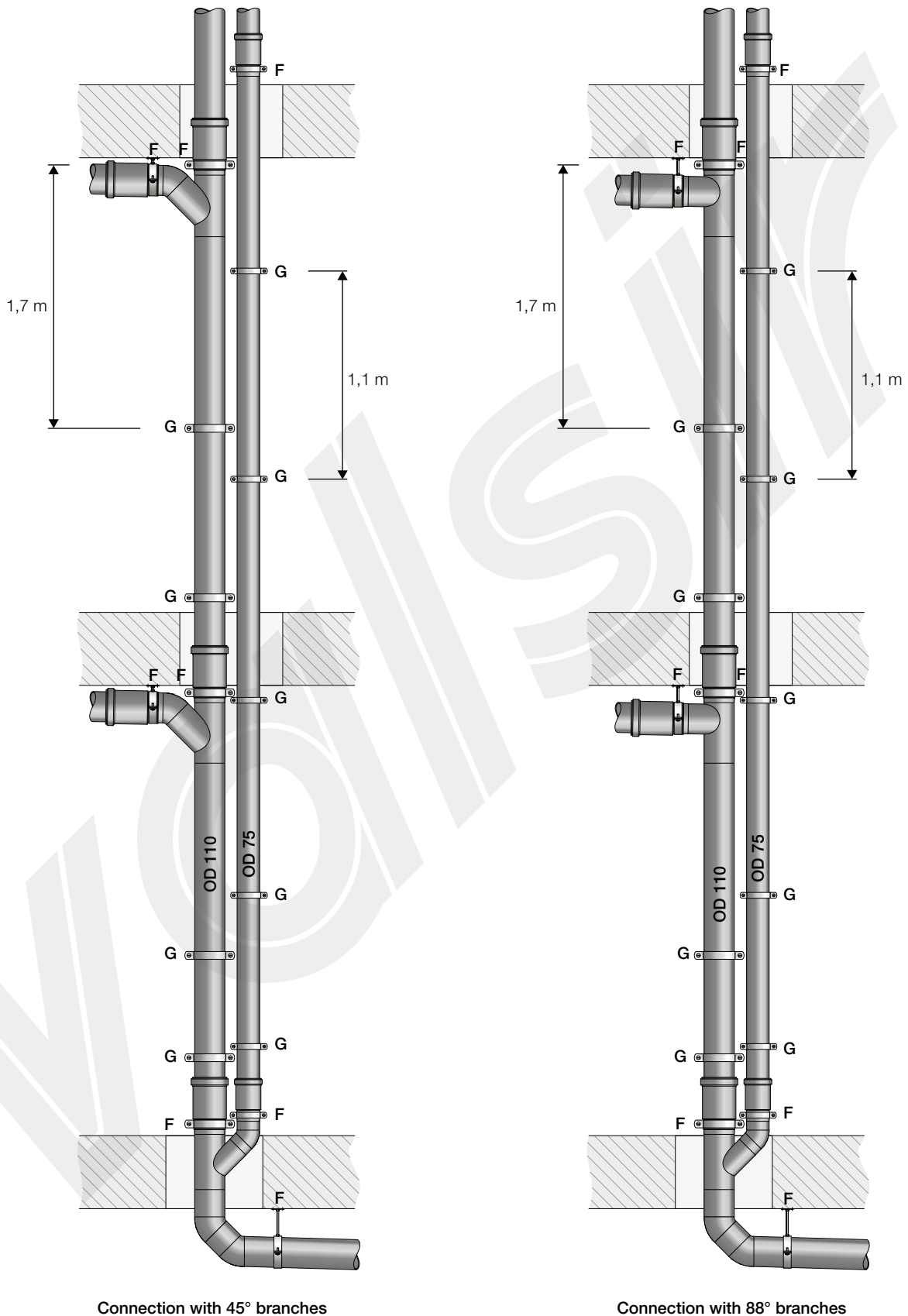
Figure 7.31 Stack OD=110 mm with parallel ventilation OD=75 mm (for HDPE).
