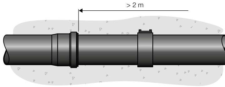
Figure 7.8 Laying in concrete of Valsir® HDPE pipe, push-fit ring seal socket.
