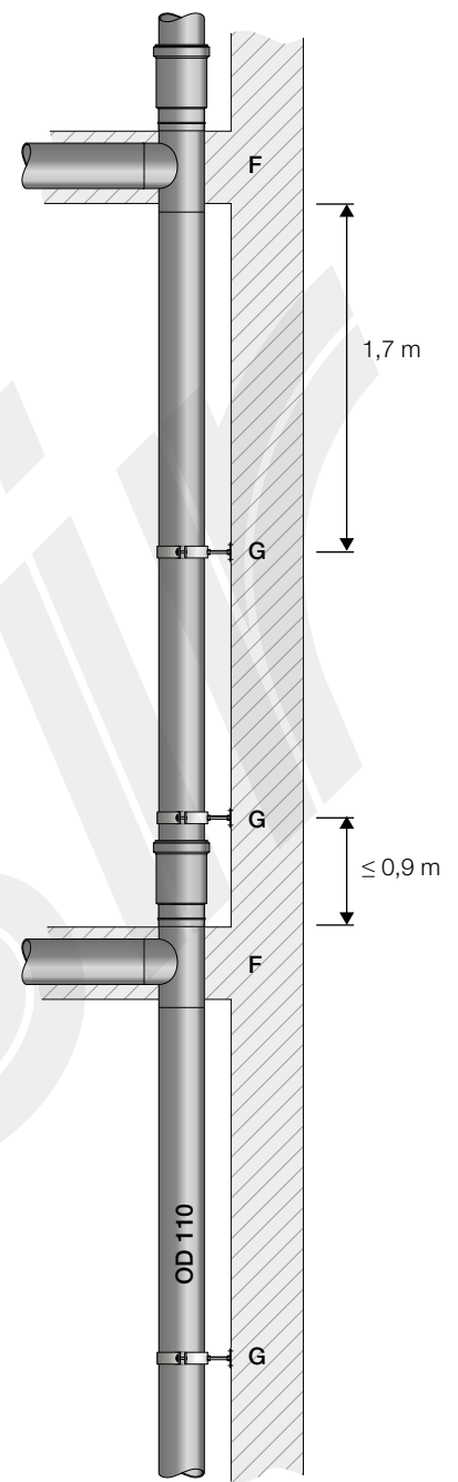
Figure 7.30 Stack OD=110 mm with inlet branches embedded in the slab (for HDPE).
