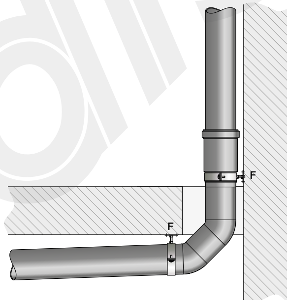
Figure 7.19 Anchor points in the presence of direction changes (for HDPE).
