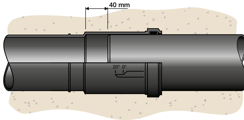
Figure 7.4 Application of expansion socket on underground pipe.
