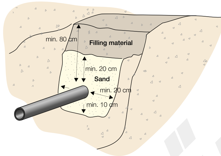
Figure 7.1 Laying of pipe in the trench, transit of light loads.
