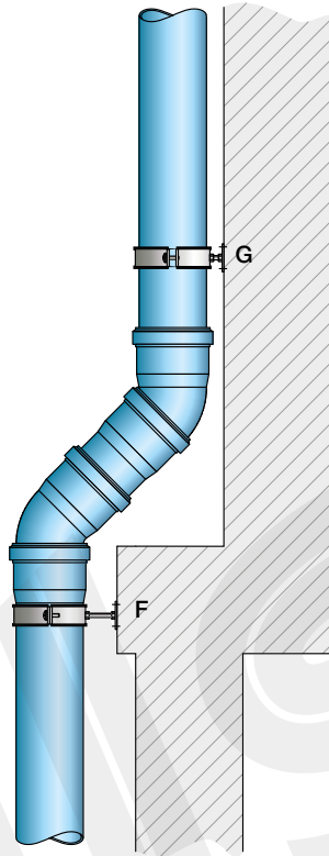
Figure 7.38 Deviation (for PP/PP3, Triplus® and Silere®).
