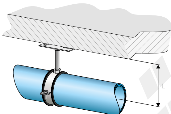
Figure 7.35 Installation distance on wall or ceiling (for PP/PP3, Triplus® and Silere®).
