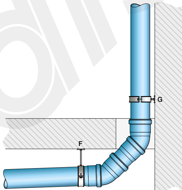
Figure 7.37 Anchor point in the presence of direction changes (for PP/PP3, Triplus® and Silere®).
