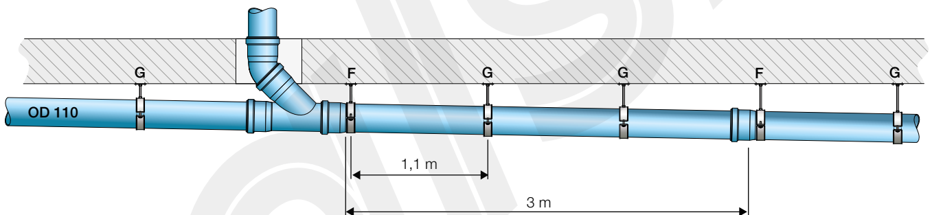
Figure 7.43 Horizontal collector pipe OD=110 mm composed of 3 m length pipes (for PP/PP3, Triplus® and Silere®).
