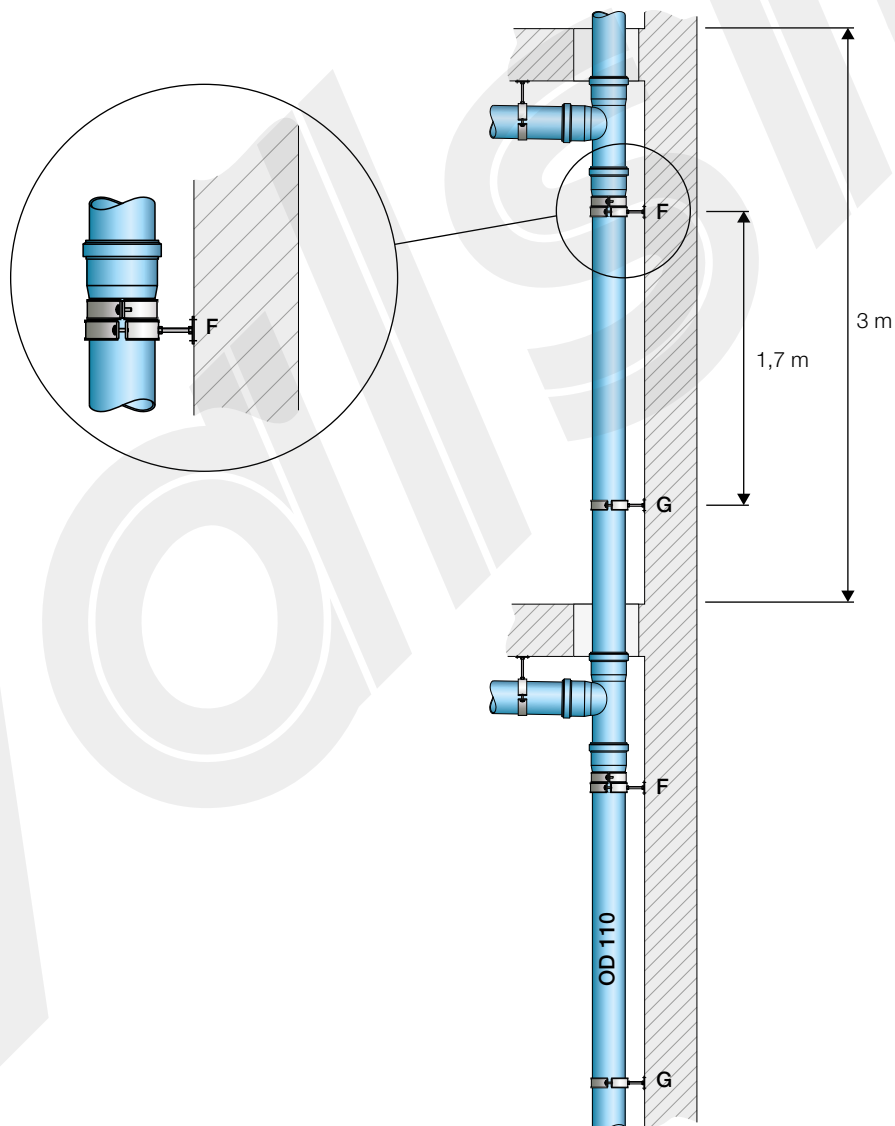
Figure 7.46 OD=110 mm stack with high performance acoustic anchor points (for Triplus® and Silere®).
