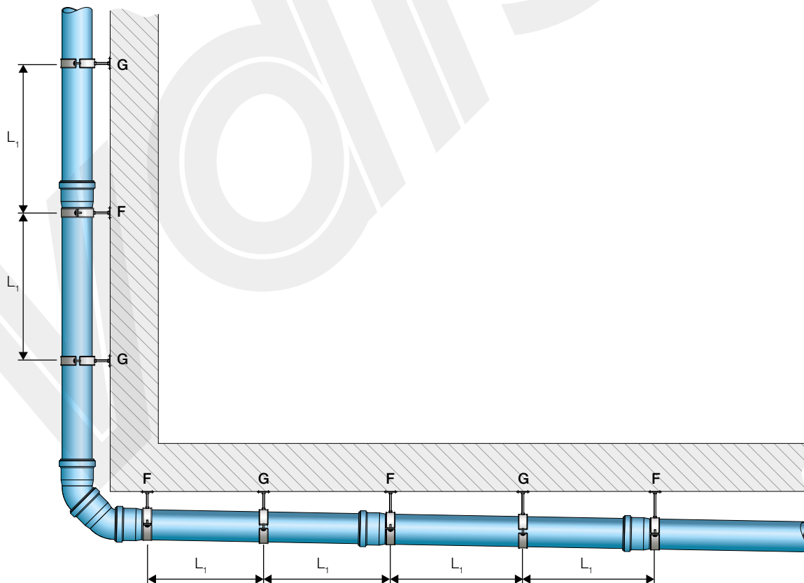
Figure 7.34 Installation using push-fit sockets (for PP/PP3, Triplus® and Silere®).
