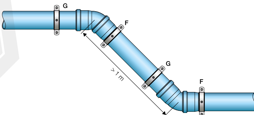
Figure 7.40 Anchor points on deviations that are greater than 1 m (for PP/PP3, Triplus® and Silere®).
