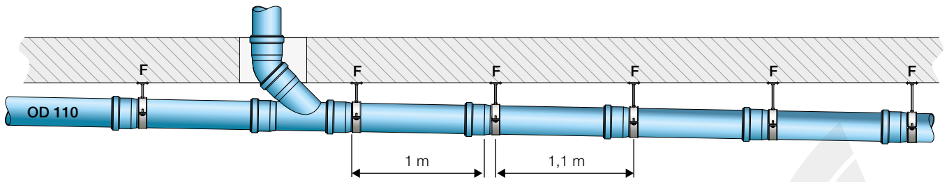
Figure 7.41 Horizontal collector pipe OD=110 mm composed of 1 m length pipes (for PP/PP3, Triplus® and Silere®).
