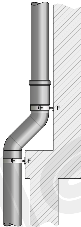
Figure 7.24 Anchor points on deviations smaller than or equal to 1 m (for HDPE).
