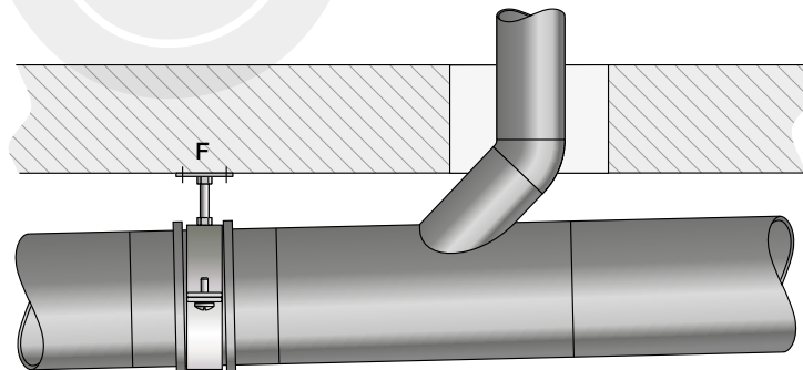
Figure 7.22 Creation of a fixed point on large diameter pipes using a double flange bushing (for HDPE).
