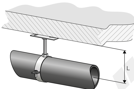
Figure 7.58 Distance of ceiling or wall installation (for HDPE).
