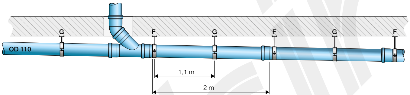
Figure 7.42 Horizontal collector pipe OD=110 mm composed of 2 m length pipes (for PP/PP3, Triplus® and Silere®).
