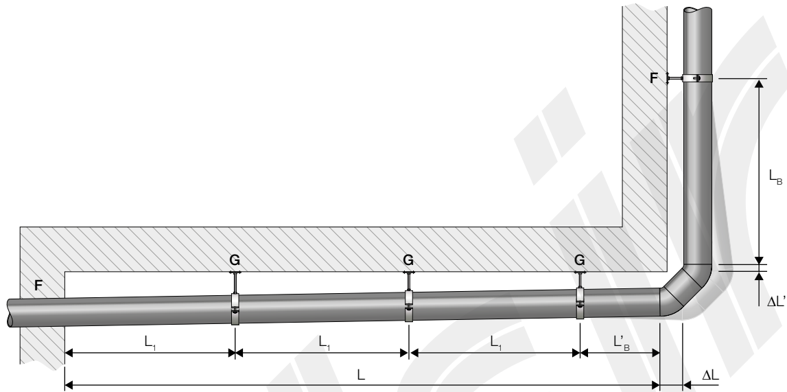
Figure 7.50 Compensation with flexible arm Type L (for HDPE).
