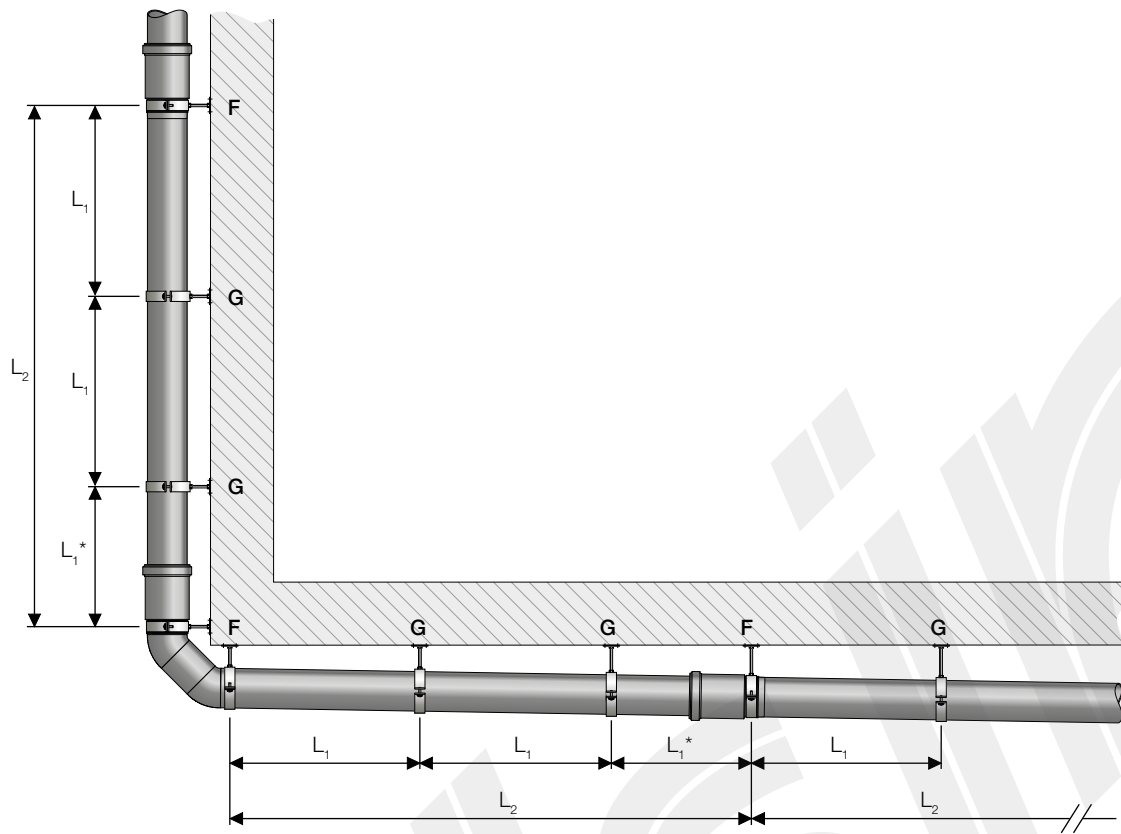
Figure 7.16 Installation using expansion sockets (for HDPE).
