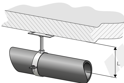
Figure 7.17 Installation distance from ceiling or wall (for HDPE).
