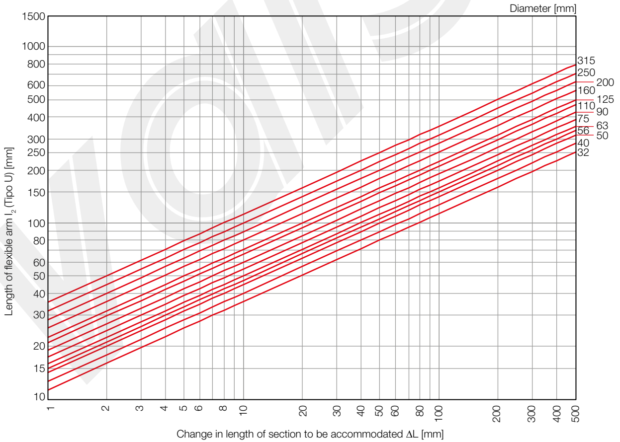
Figure 7.56 Calculation of the length of arm l_2 of the “omega” Type U (for HDPE).
