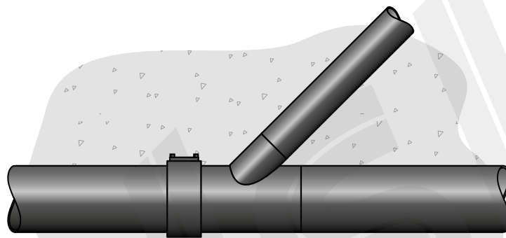
Figure 7.6 Laying in concrete of Valsir® HDPE pipe, electrofusion coupling as fixed point.
