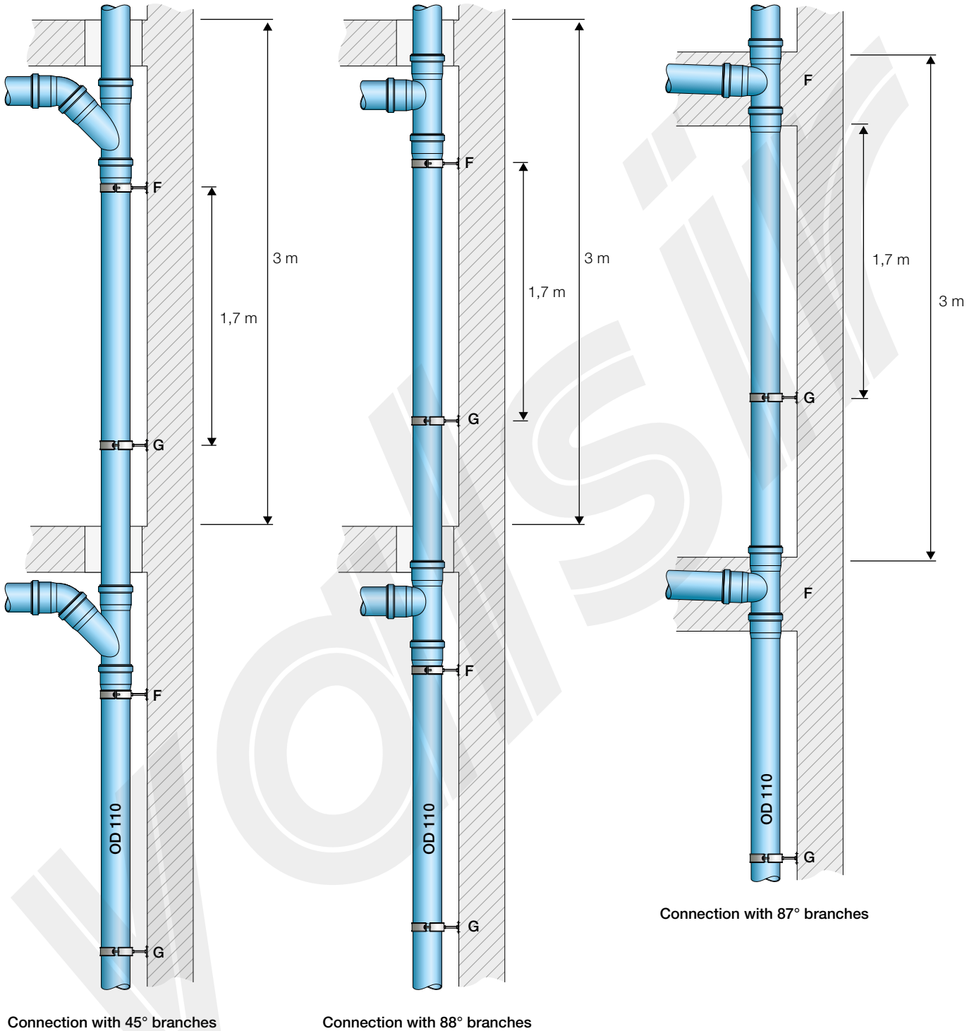
Figure 7.45 OD=110 mm stack with inlet branches embedded in the slab (for PP/PP3, Triplus® and Silere®).
