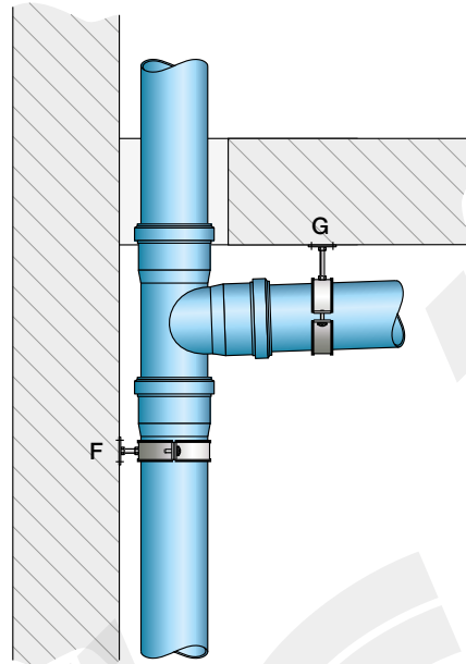
Figure 7.36 Anchor point in the presence of a branch (for PP/PP3, Triplus® and Silere®).
