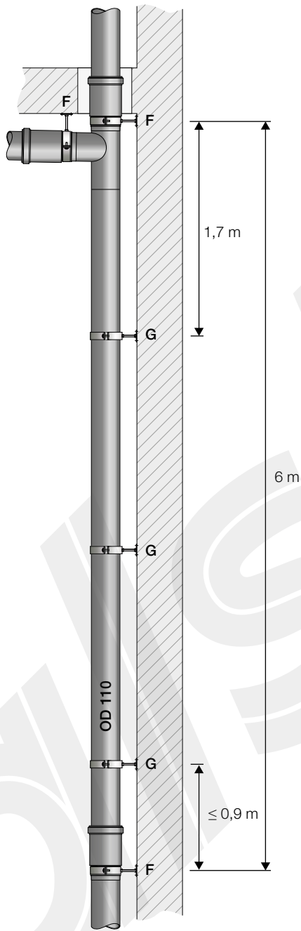
Figure 7.29 Stack OD=110 mm with inlet branches at intervals greater than 6 m (for HDPE).
