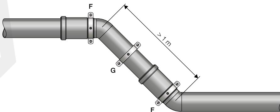
Figure 7.25 Anchor points on deviations greater than 1 m (for HDPE).
