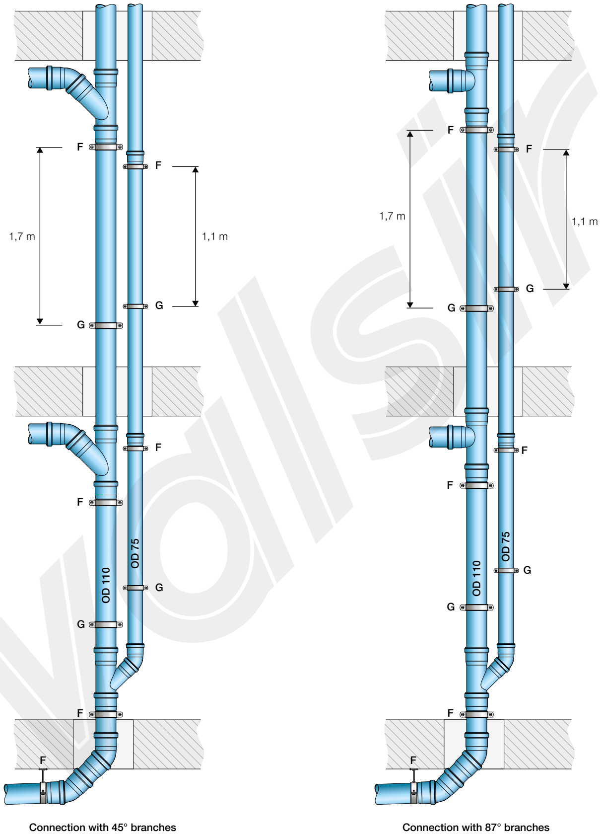
Figure 7.47 OD=110 mm stack with parallel ventilation OD=75 mm (for PP/PP3, Triplus® and Silere®).
