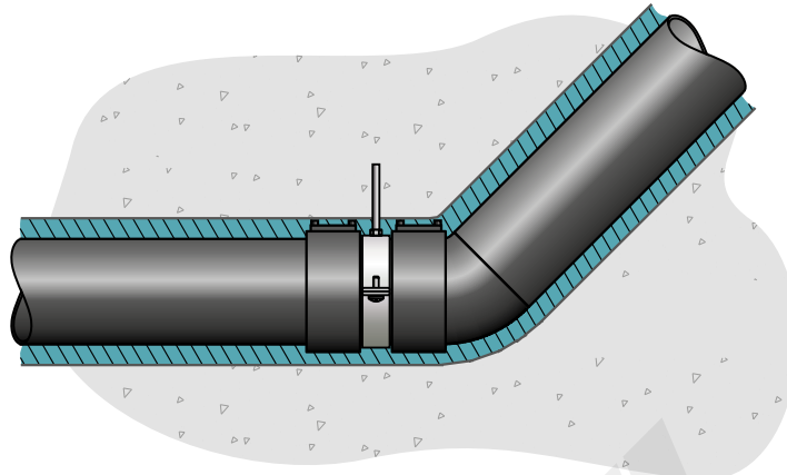
Figure 7.5 Laying in concrete of Valsir® HDPE pipe with lagging.
