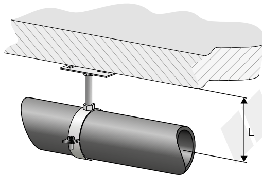
Figure 7.49 Ceiling or wall installation distance (for HDPE).
