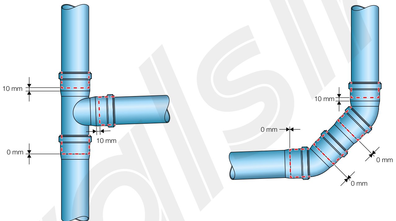
Figure 7.33 Examples of a correct use of the push-fit socket (for PP/PP3, Triplus® and Silere®).
