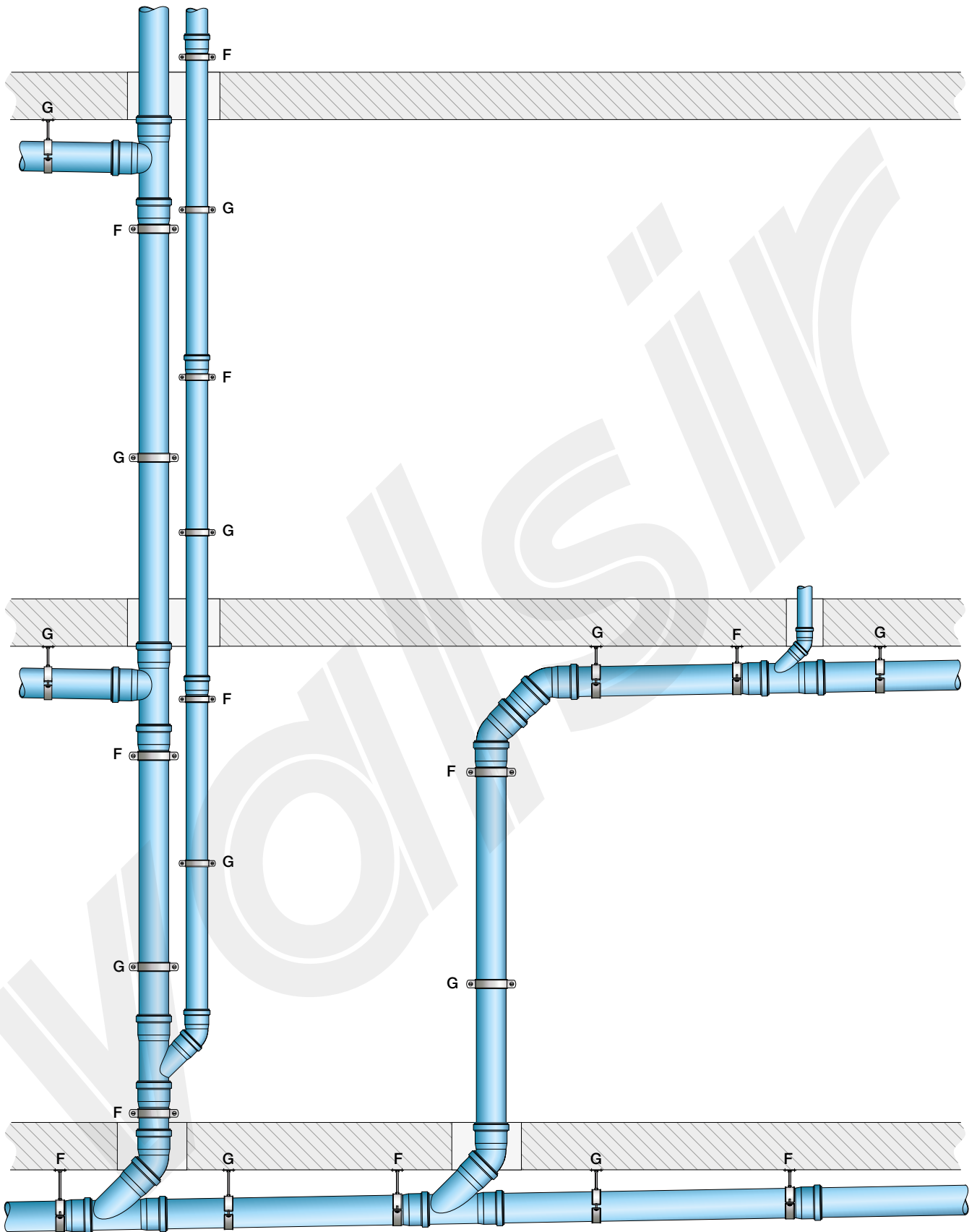
Figure 7.48 Example of system layout (for PP/PP3, Triplus® and Silere®).
