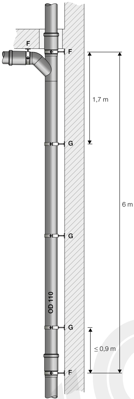
Figure 7.29 Stack OD=110 mm with inlet branches at intervals greater than 6 m (for HDPE).
