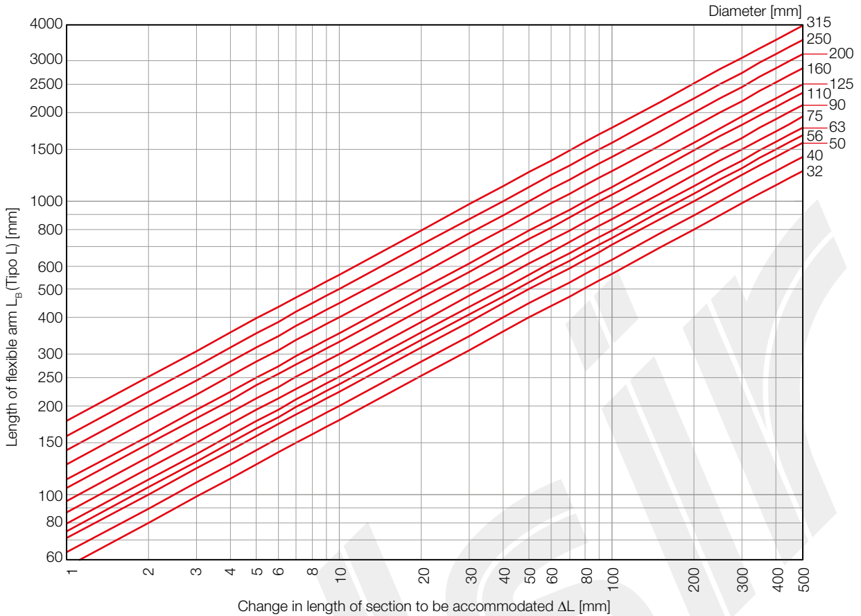
Figure 7.51 Calculation of compensation length using flexible arm Type L (for HDPE).
