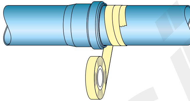
Figure 7.9 Laying in concrete, protection of push-fit ring seal socket.
