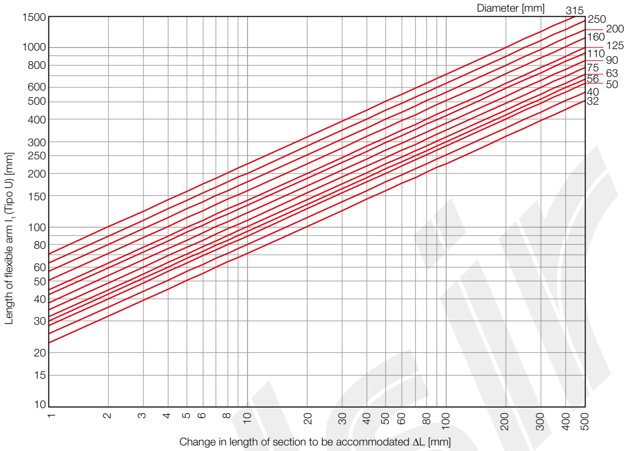
Figure 7.55 Calculation of the length of the arm l_1 of the “omega” Type U (for HDPE).
