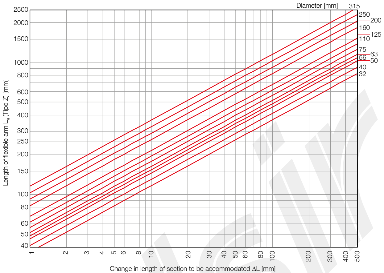
Figure 7.53 Calculation of the compensation length using flexible arm disalignment Type Z (for HDPE).
