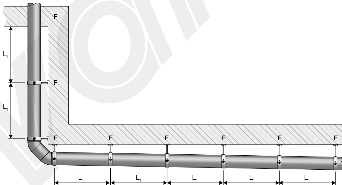
Figure 7.57 Rigid installation using fixed point brackets (for HDPE).
