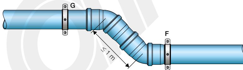
Figure 7.39 Anchor points on deviations that are smaller than or equal to 1 m (for PP/PP3, Triplus® and Silere®).
