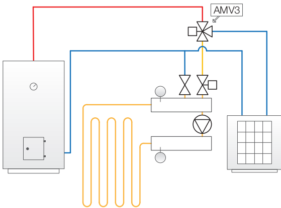
Figure 02. Switching valve in heating- or cooling system.
