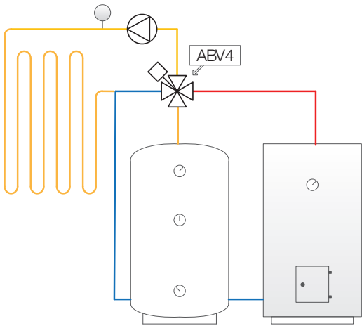
Figure 02. Mixing valve in underfloor- or radiator heating system that automatically combines different heat sources.
