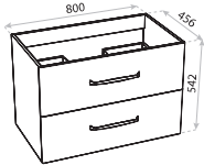
UMYWALKA WASHBASIN NEVADA 80
