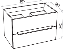
UMYWALKA WASH-BASIN KANSAS 80
