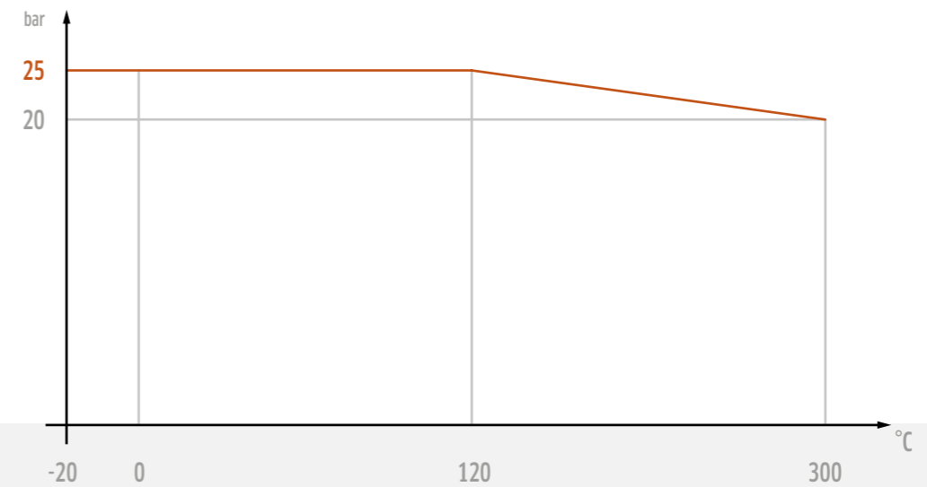
Diagram: pressure / temperature ratio
